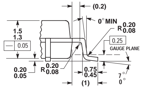
VIEW AA
