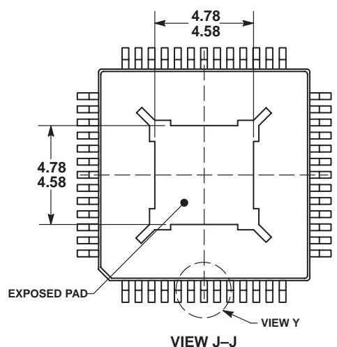
VIEW J-J
